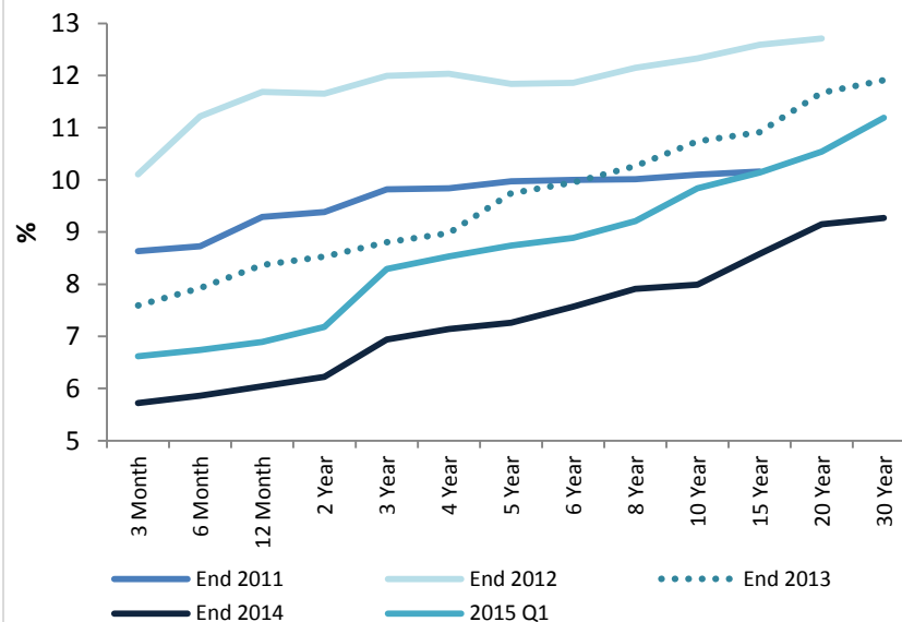
Secondary Market Yield Curve
