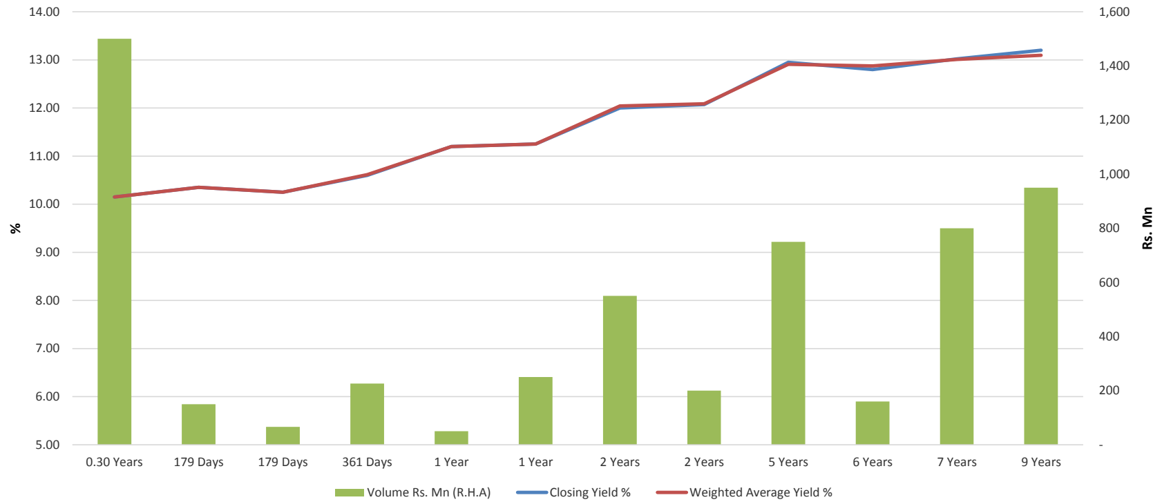
Yield Curve and Trade Volume 24.03.2017
