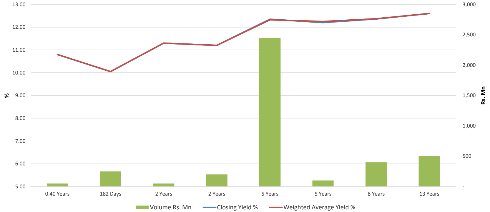
Yield Curve and Trade Volume 18.01.2017
