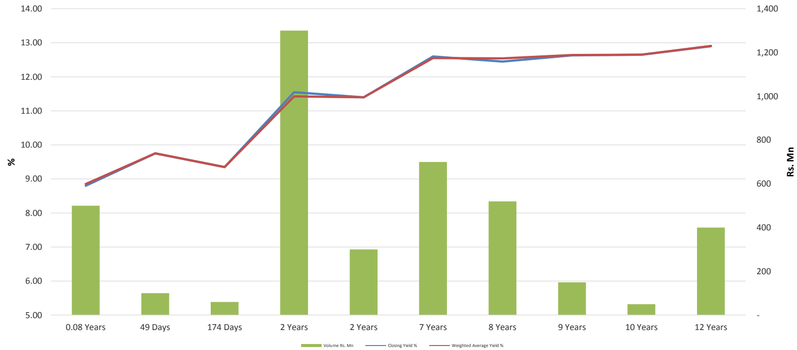
Yield Curve and Trade Volume 15.12.2016
