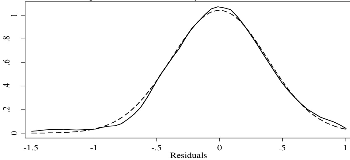
Figure A2: Kernel Density Estimate of Residuals
