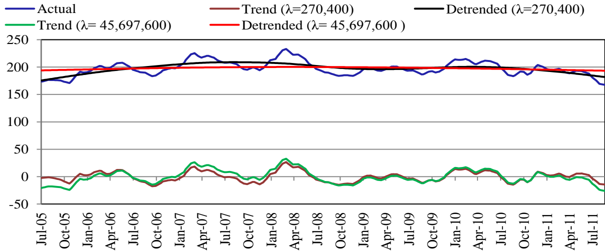
Figure A1: Detrending of IIP Series
