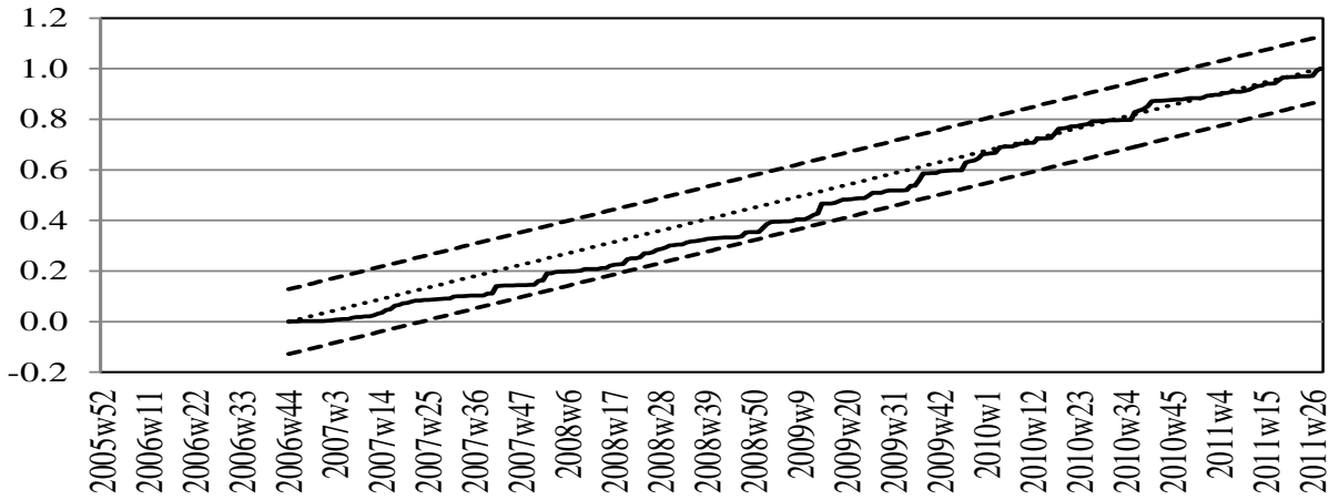
CUSUM SQUARE Test Statistics with 95 % Confidence Interval
